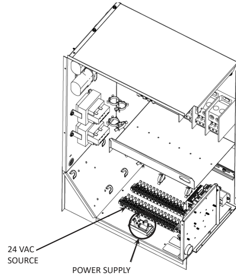
Figure 6 - Medium Chassis
